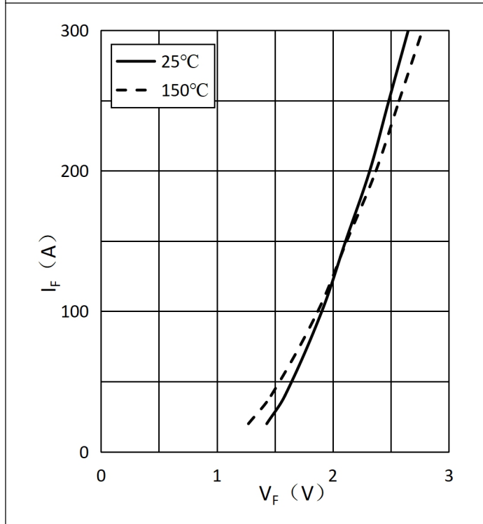
I_F = f(V_F) Fig.7 Typ. Forward Characteristics of Diode-Inverter 图 7 二极管正向偏压特性-逆变器
