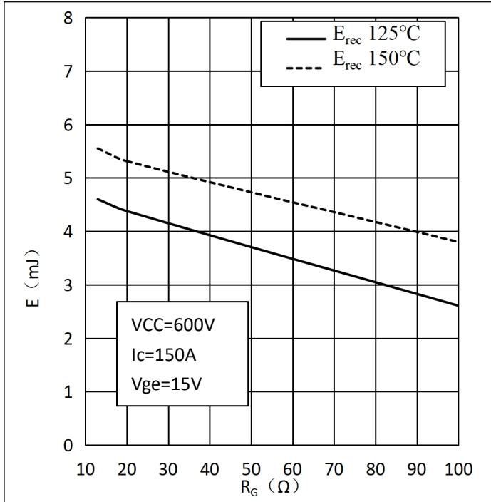
Fig.9 Switching Loss of Diode vs. Gate Resistor-Inverter
