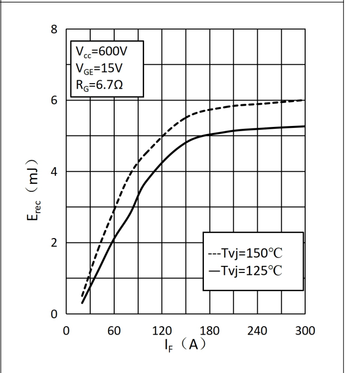
E_{rec} = f(I_F) Fig.8 Typ. Switching Losses of Diode-Inverter 图 8 二极管开关损耗-逆变器
