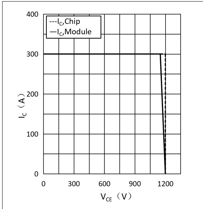
I_c = f(V_{CE}) Fig.5 Reverse Bias Safe Operating Area (RBSOA) -Inverter 图 5 反偏安全工作区-逆变器
