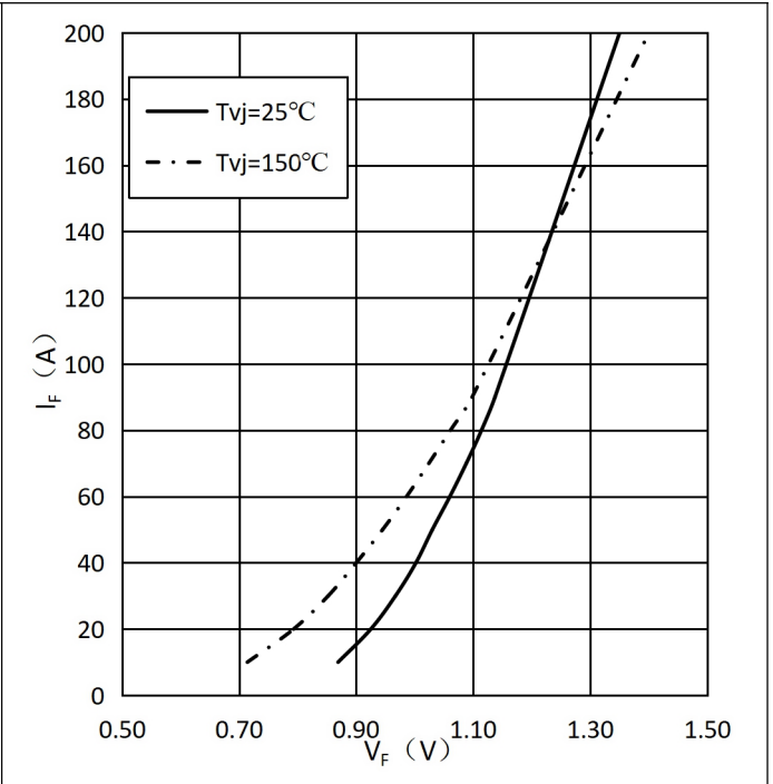
Fig.10 Forward Characteristics of Diode-Rectifier
