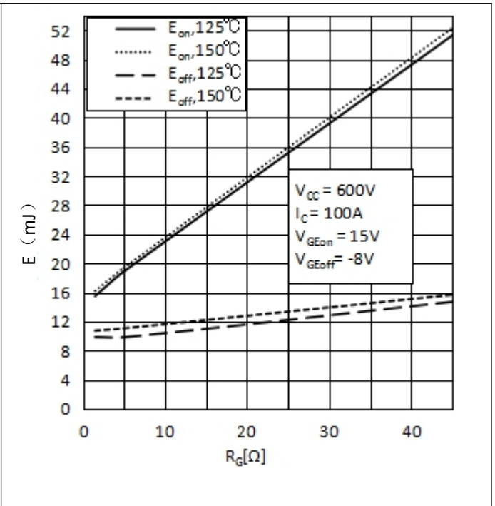
E_{on} = f(R_G) , E_{off} = f(R_G) Fig.6 Switching Loss of IGBT vs. Gate Resistor - Inverter 图 6 IGBT 开关损耗和门极电阻-逆变器
