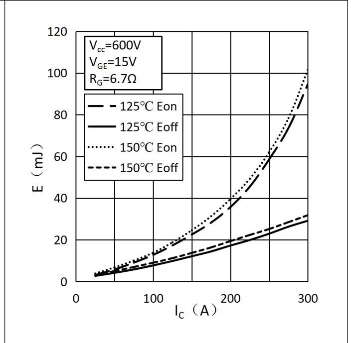
E_{on}=f(I_c), E_{off}=f(I_c) Fig.4 Switching Loss vs. Collector Current-Inverter 图 4 开关损耗和集电极电流-逆变器
