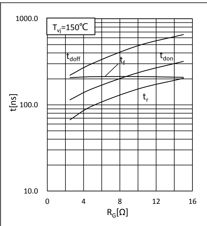
V_{CC} = 350\text{ V} , I_C = 400\text{ A} , V_{GE} = -8/15\text{ V} , T_{vj} = 150^\circ\text{C} Fig.6: Switching Times vs. Gate Resistor 图 6: 开关时间与门极电阻关系
