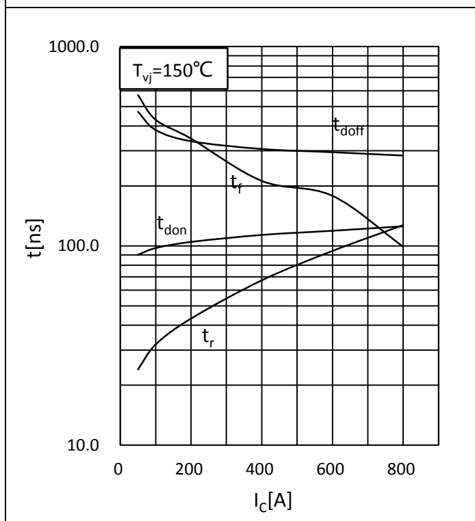
V_{CC} = 350\text{ V} , V_{GE} = 15\text{ V} , R_G = 2.5\ \Omega , T_{vj} = 150^\circ\text{C} Fig.7: Switching Times vs. I_c 图 7: 开关时间与集电极电流关系
