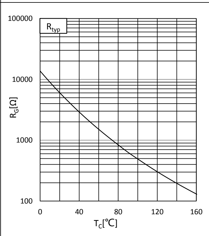
Fig.12: Typ. NTC-Temperature Characteristics
