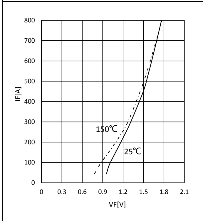
I_F = f(V_F) Fig.3: Forward characteristic 图 3: 正向特性
