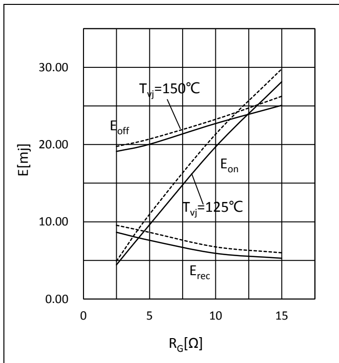
V_{GE} = 15\text{ V} , I_C = 400\text{ A} , V_{CE} = 350\text{ V} Fig.5: Switching Loss vs. Gate Resistor 图 5: 开关损耗与门极电阻关系
