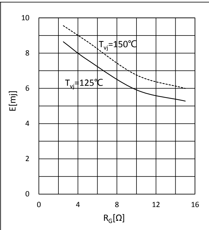
Fig.10: Reverse recovery Energy vs. Gate Resistor
