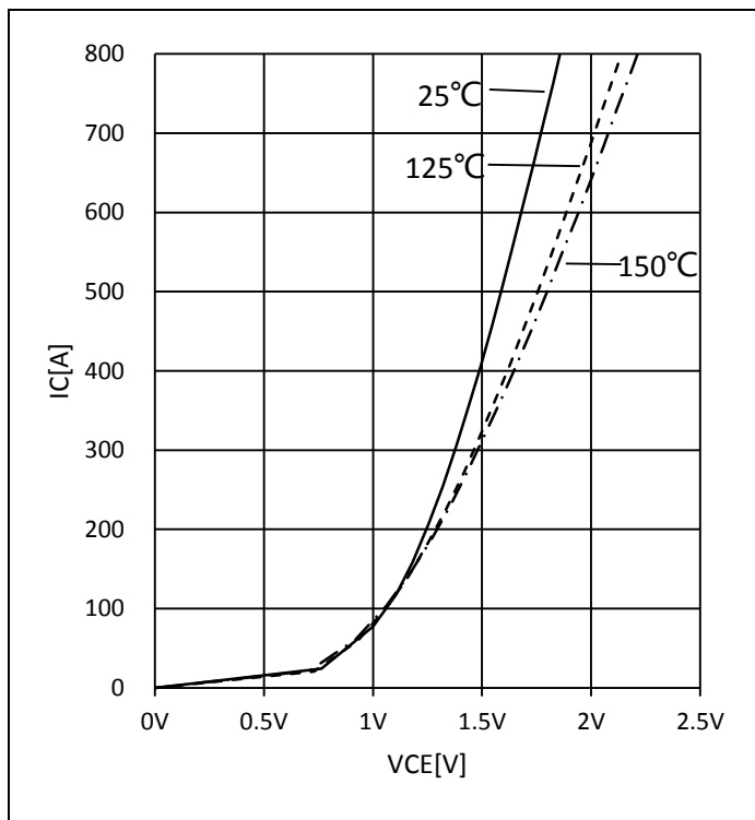
V_{GE} = 15V, I_C = f(V_{CE}) Fig.1: On-state Characteristics 图 1: 通态特性
