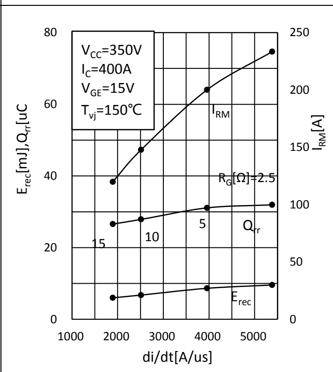
V_{CC} = 350\text{ V} , I_C = 400\text{ A} , V_{GE} = 15\text{ V} , T_{vj} = 150^\circ\text{C} Fig.8: Reverse recovery characteristics vs. di/dt 图 8: 反向恢复特性
