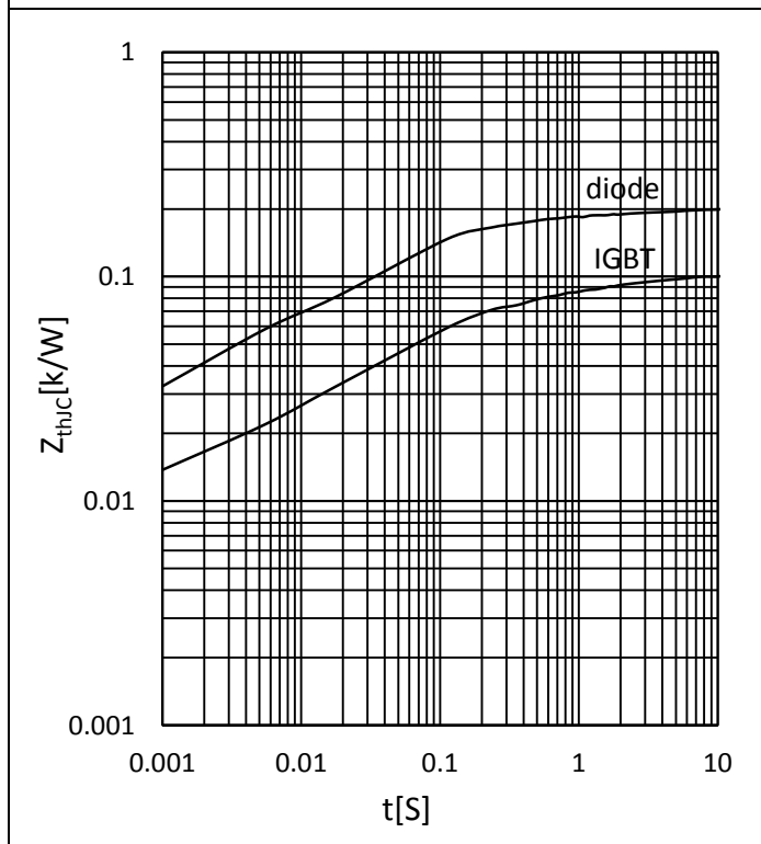
Fig.11: Typ. transient thermal impedance
