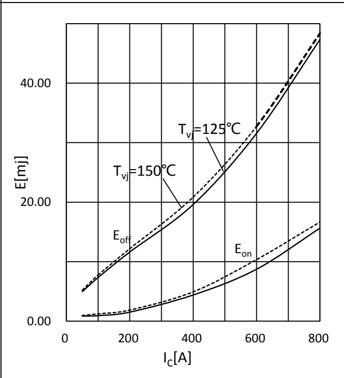
V_{GE} = 15V, R_{Gon} = 2.5 \Omega, R_{Goff} = 5 \Omega, V_{CE} = 350V Fig.4: Switching Loss vs. Collector Current 图 4: 开关损耗与集电极电流关系
