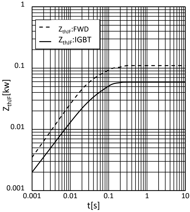
Fig.9 Transient Thermal Impedance
