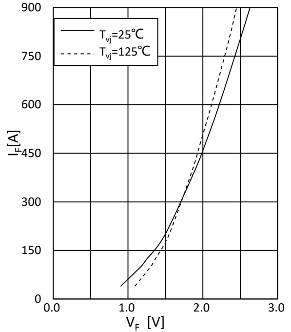
Fig.6 Forward Characteristics
