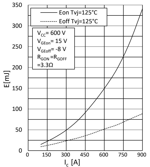
Fig.4 Switching Loss vs. Collector Current 图 4 开关损耗和集电极电流
