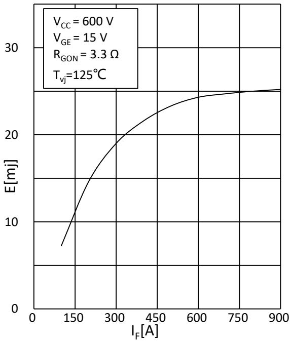
Fig.7 Reverse recovery Energy
