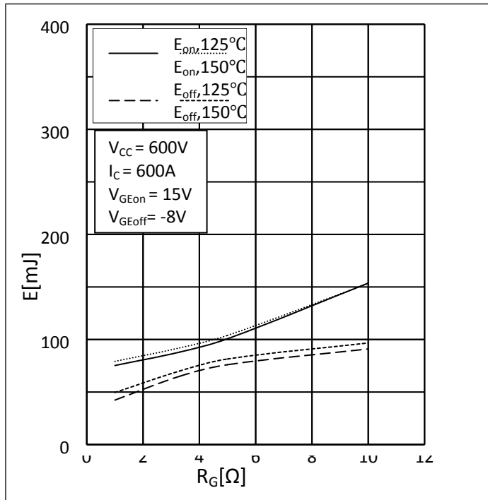
Fig.5: Switching Loss vs. Gate Resistor 图 5: 开关损耗与门极电阻关系
