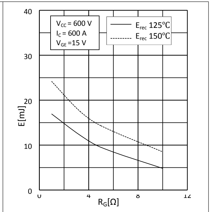
Fig.10: Reverse recovery Energy vs. Gate Resistor
