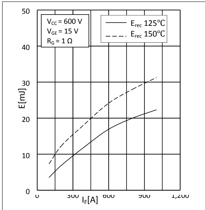
Fig.9: Reverse recovery Energy
