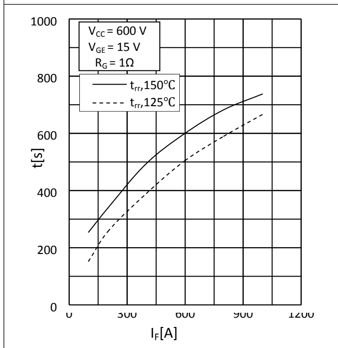
Fig.11: Reverse Recovery Times vs. I_F
