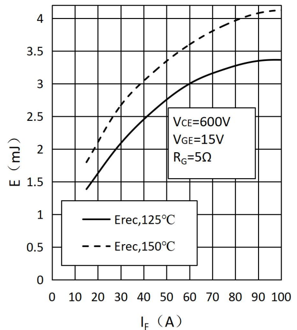
Fig.8 Typ. Switching Losses of Diode-Inverter 图 8 二极管开关损耗-逆变器
