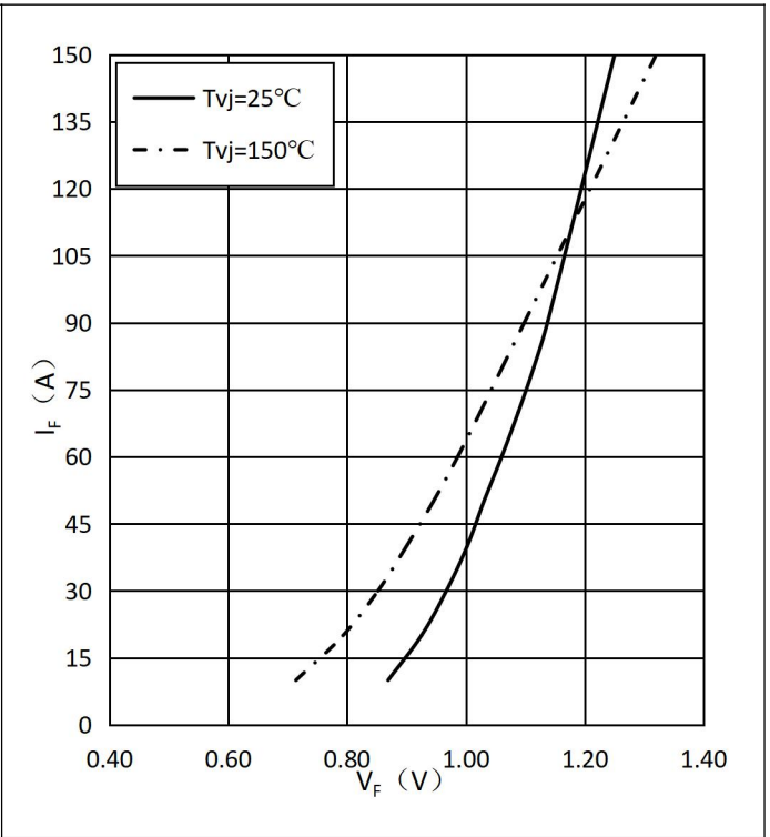
Fig.10 Forward Characteristics of Diode-Rectifier
