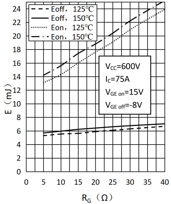
Fig.6 Switching Loss of IGBT vs. Gate Resistor - Inverter
