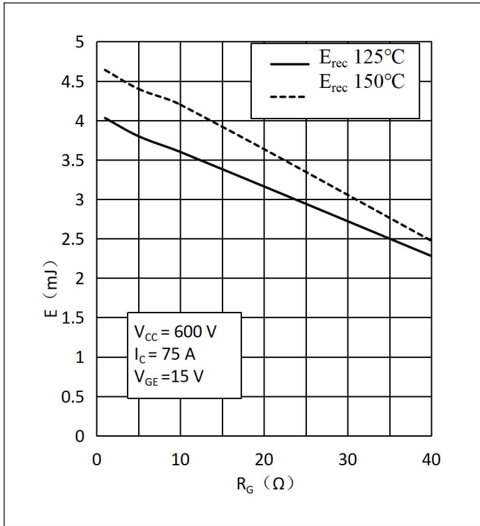
Fig.9 Switching Loss of Diode vs. Gate Resistor -Inverter
