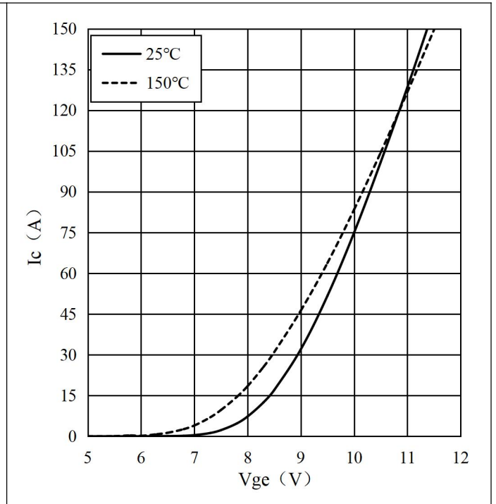
Fig.2 Typ. Transfer Characteristics-Inverter
