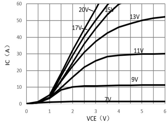
Figure 2. Typical output characteristic( T_j=150^{\circ}\text{C} )
