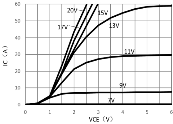
Figure 1. Typical output characteristic( T_j=25^{\circ}\text{C} )
