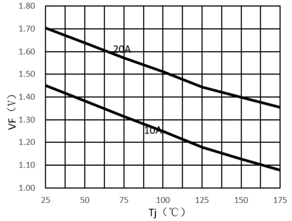
Figure 4. V_F vs. T_j
