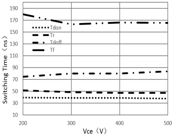
Figure 9. Switching times vs V_{CE} ( T_j=150^\circ C, V_{GE}=15V, I_C=20A, R_G=10\Omega )
