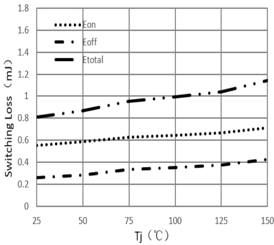
Figure 7. Switching energy losses vs T_j ( V_{CE}=400V, V_{GE}=15V, I_C=20A, R_G=10\Omega )
