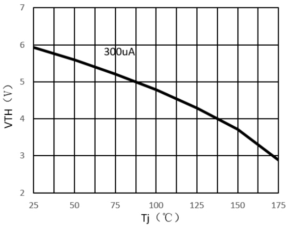
Figure 5. V_{\text{TH}} vs. T_j
