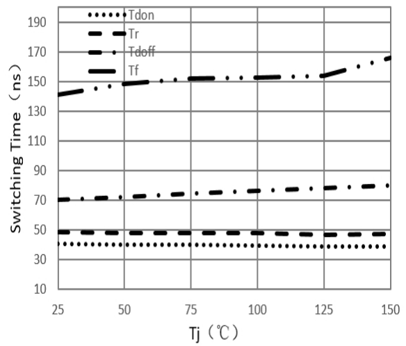
Figure 8. Switching times vs T_j ( T_j=25^\circ C, V_{GE}=15V, I_C=20A, R_G=10\Omega )
