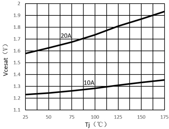
Figure 3. V_{\text{cesat}} vs. T_j
