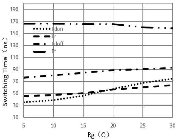
Figure 11. Switching times vs R_g ( T_j=150^\circ C, V_{CE}=400V, V_{GE}=15V, I_C=20A )
