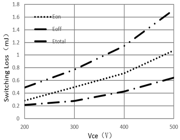
Figure 10. Switching energy losses vs V_{CE} ( T_j=150^\circ C, V_{CE}=400V, V_{GE}=15V, I_C=20A )
