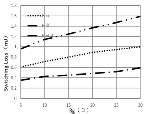
Figure 12. Switching energy losses vs R_g ( T_j=150^\circ C, V_{CE}=400V, V_{GE}=15V, I_C=20A )
