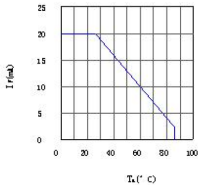
Fig.5 Maximum Forward Current vs. Ambient Temperature
