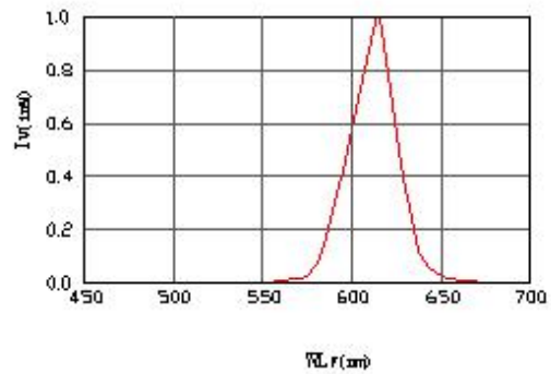
Fig.3 Relative Luminous Intensity vs. Wavelength
