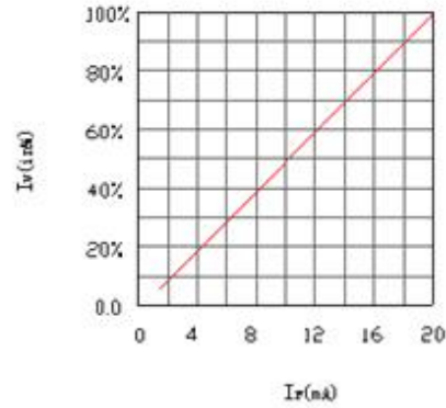
Fig.2 Relative Luminous Intensity vs. Forward Current
