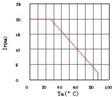
Fig.5 Maximum Forward Current vs. Ambient Temperature
