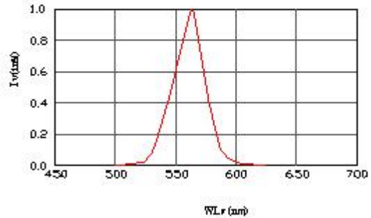
Fig.3 Relative Luminous Intensity vs. Wavelength
