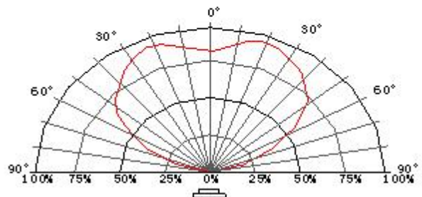
Fig.6 Relative Luminous Intensity vs. Radiation Angle
